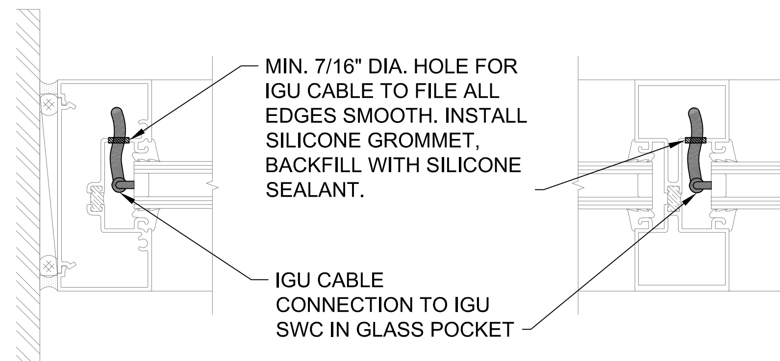
DETAIL 5 VERTICAL MULLION
